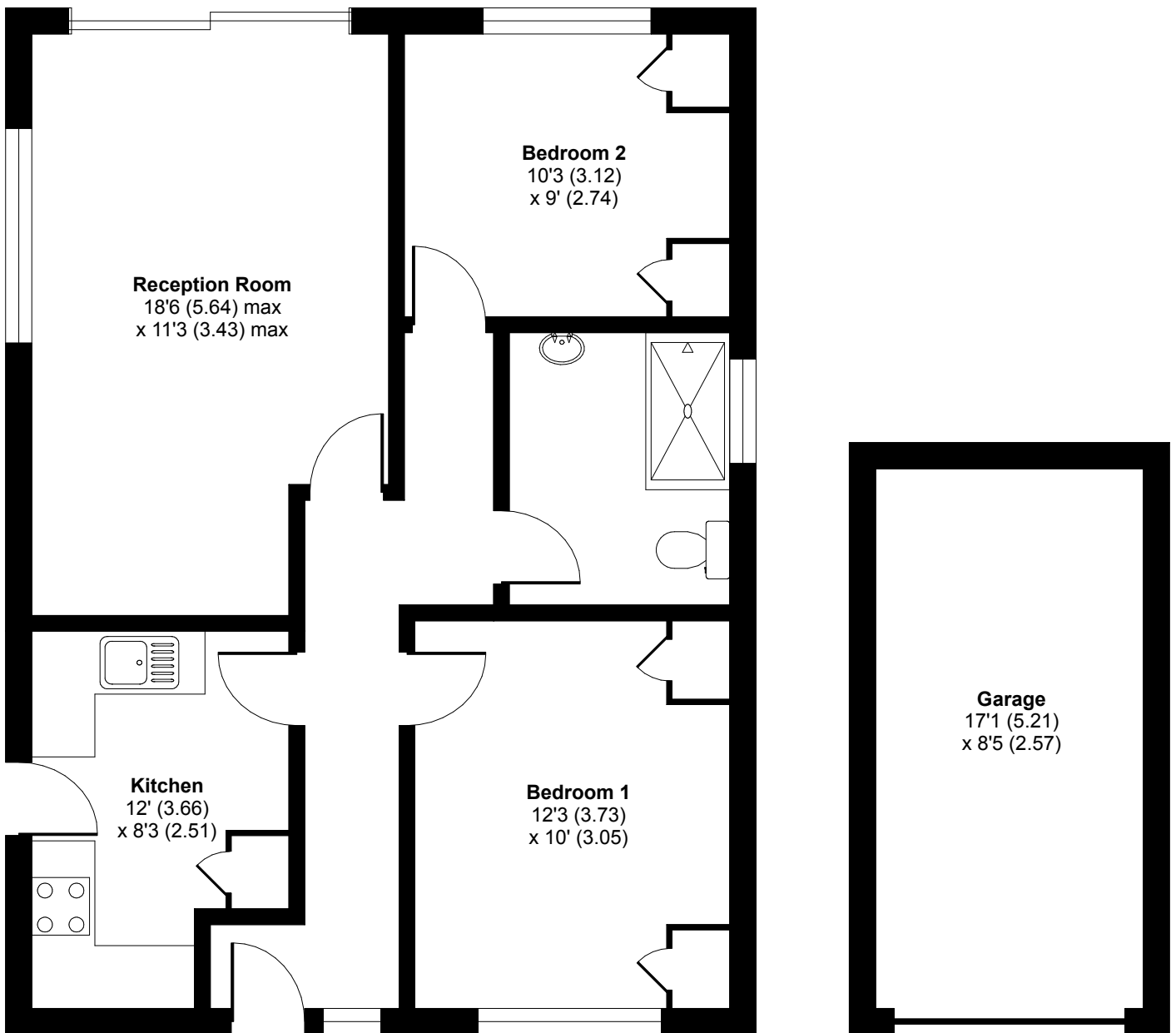
GROUND FLOOR
